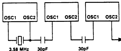
Figure 8. Common Crystal Connection
