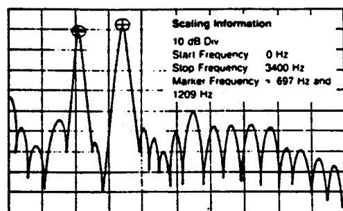
Figure 7. Spectrum Plot
