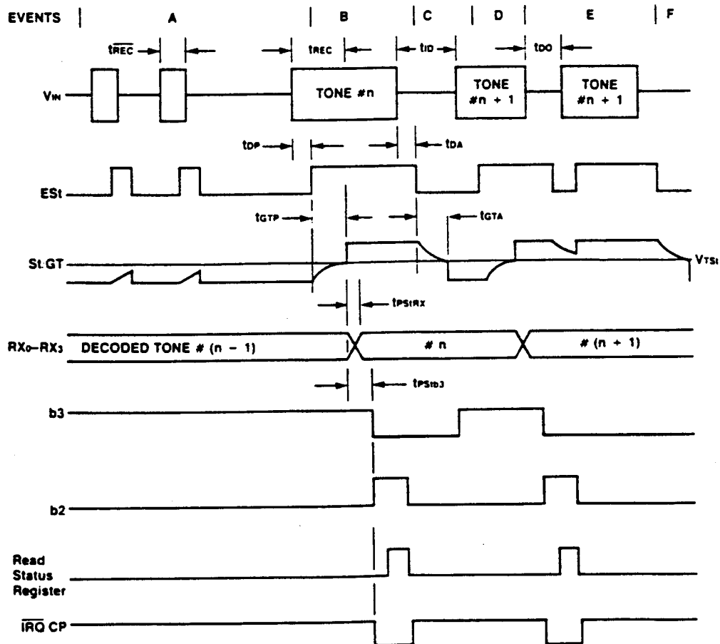
General Transceiver Timing
