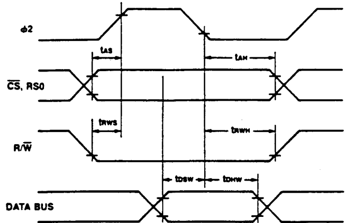
Microprocessor Write Cycle
