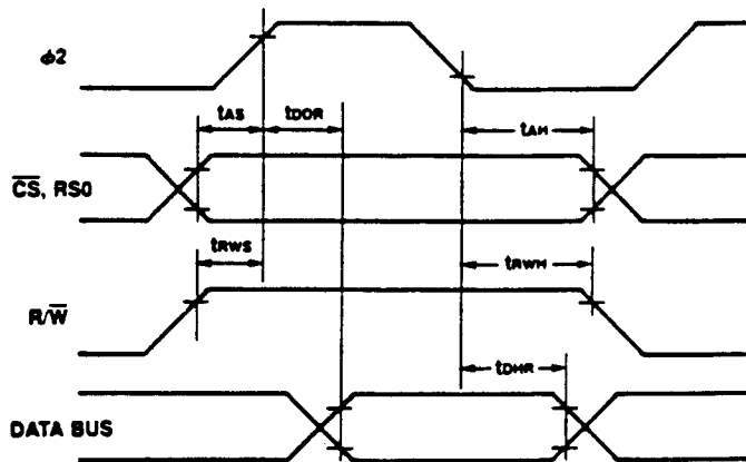
Microprocessor Read Cycle
